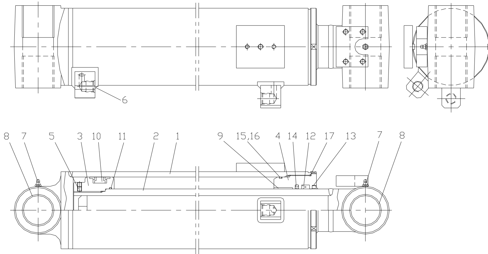
Fig. 2-2 SCK1213 DERRICK CYL'D ASS'Y
