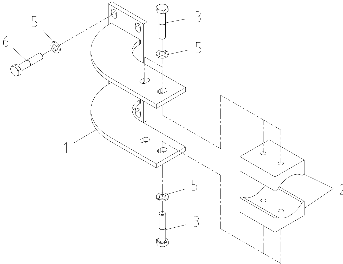
Fig. 9-3 SCK1213 EXP' CYL' GUIDE SET
