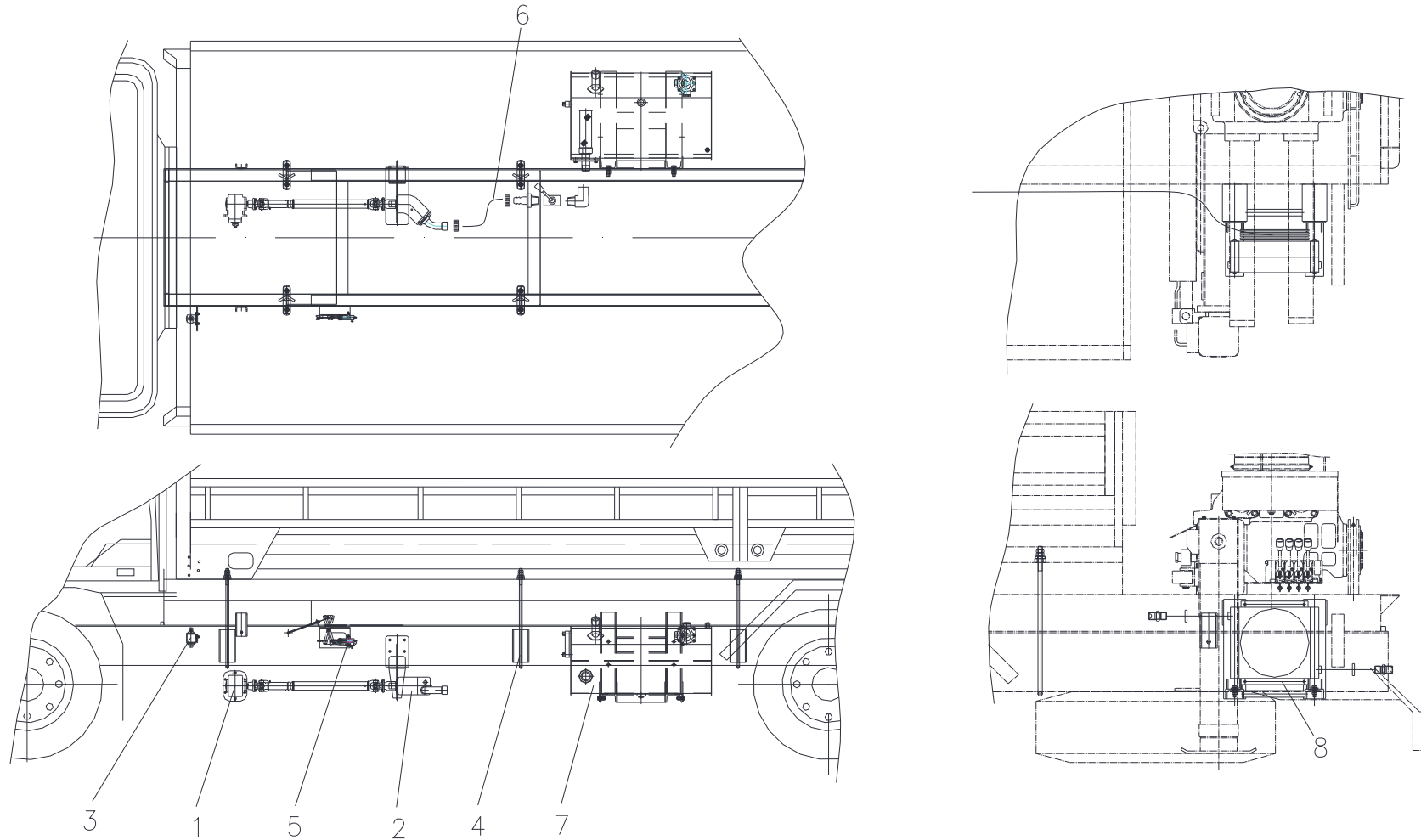
Fig. 7 SCK1213 MOUNTING ASS'Y
