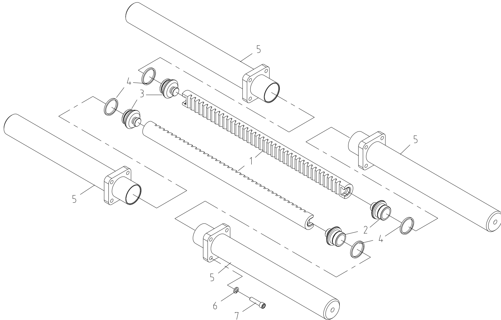
Fig. 2-1-2 SCK1213 RACK CYL'D ASS'Y
