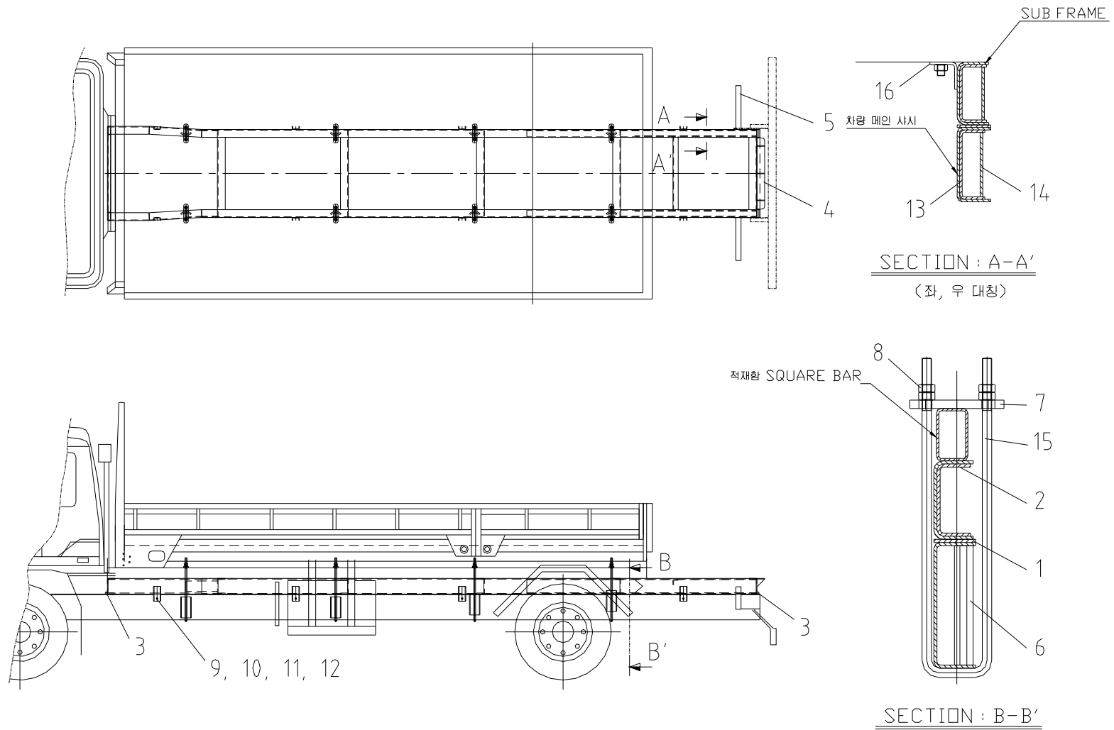
Fig. 7-3 SCK1213 MOUNTING SET
