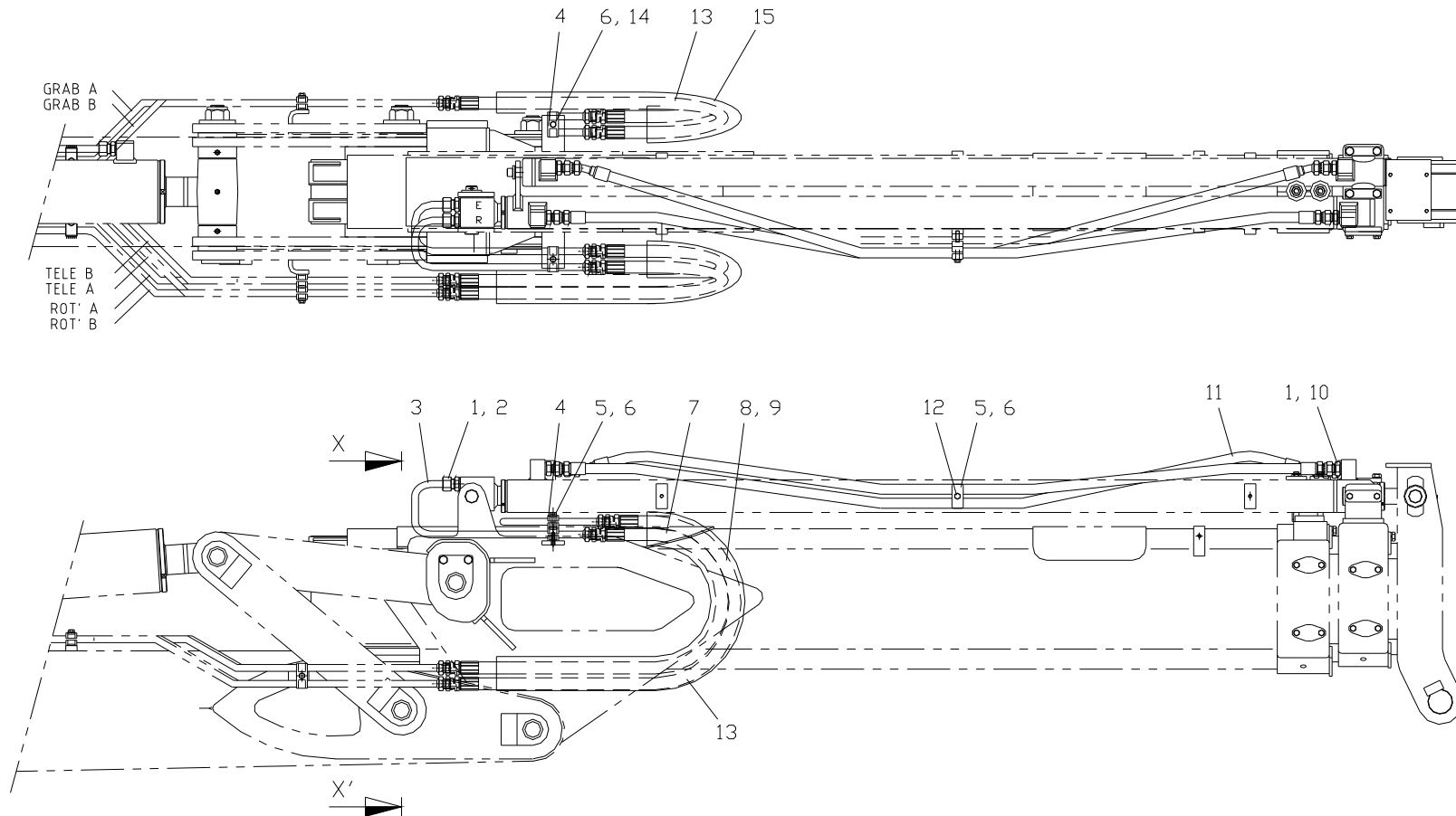
Fig. 4-7 SCK1213 TELE PIPING
