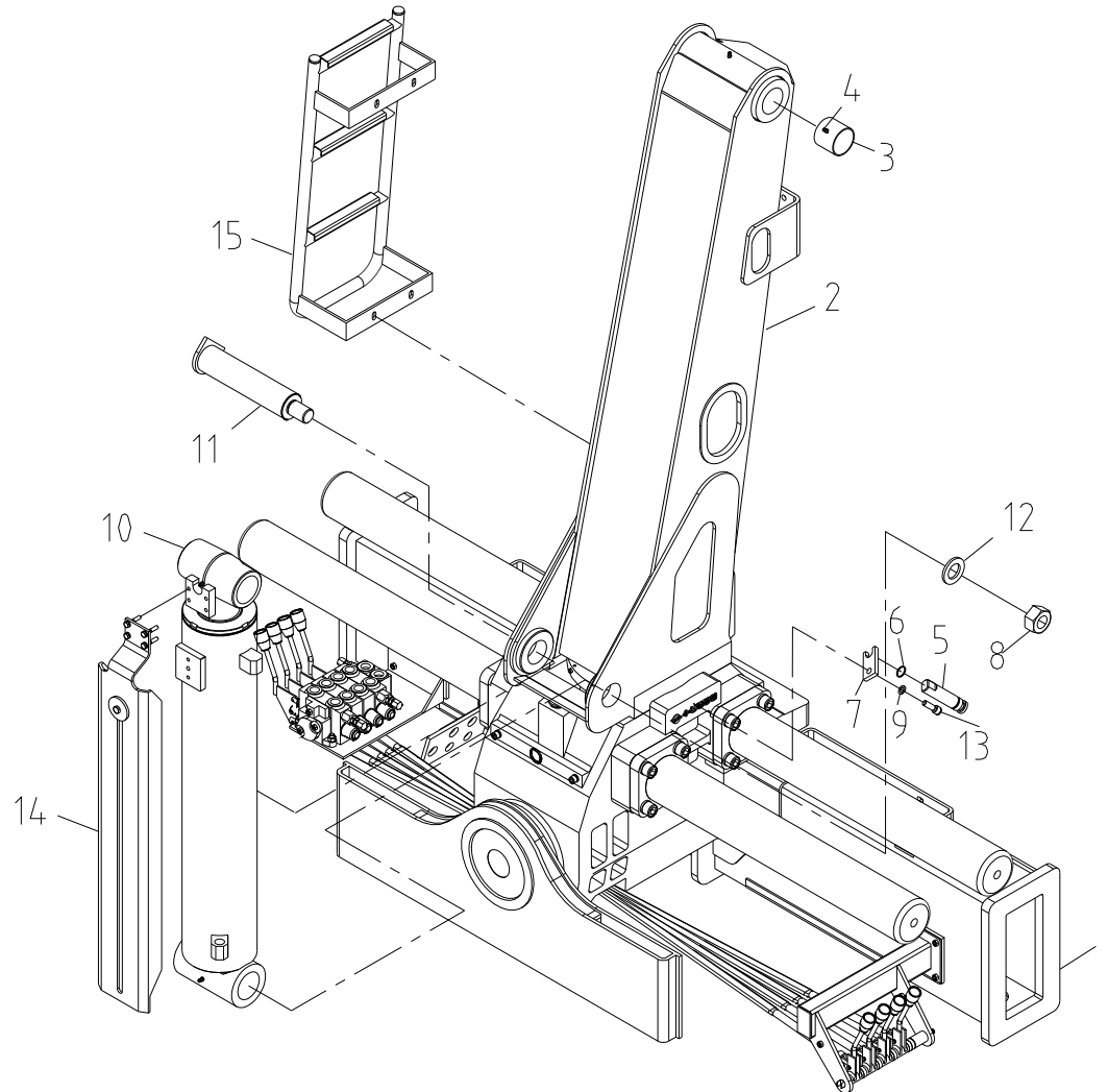
Fig. 2 SCK 1213 BASE &amp; POST ASS'Y
