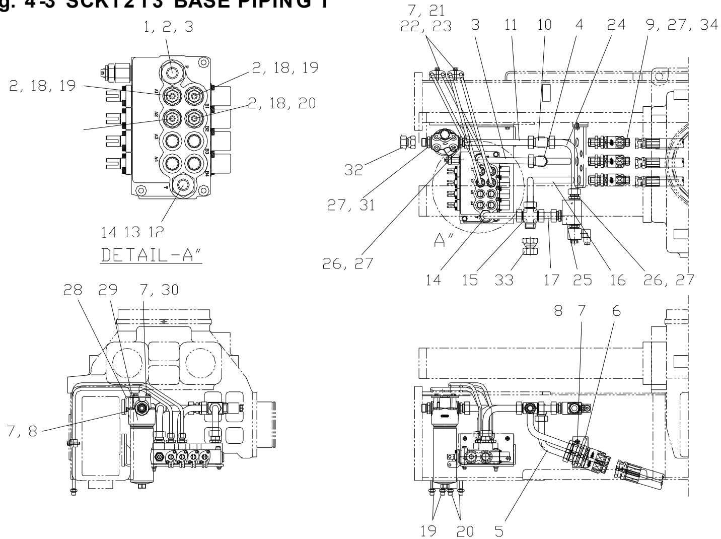
Fig. 4-3 SCK1213 BASE PIPING 1
