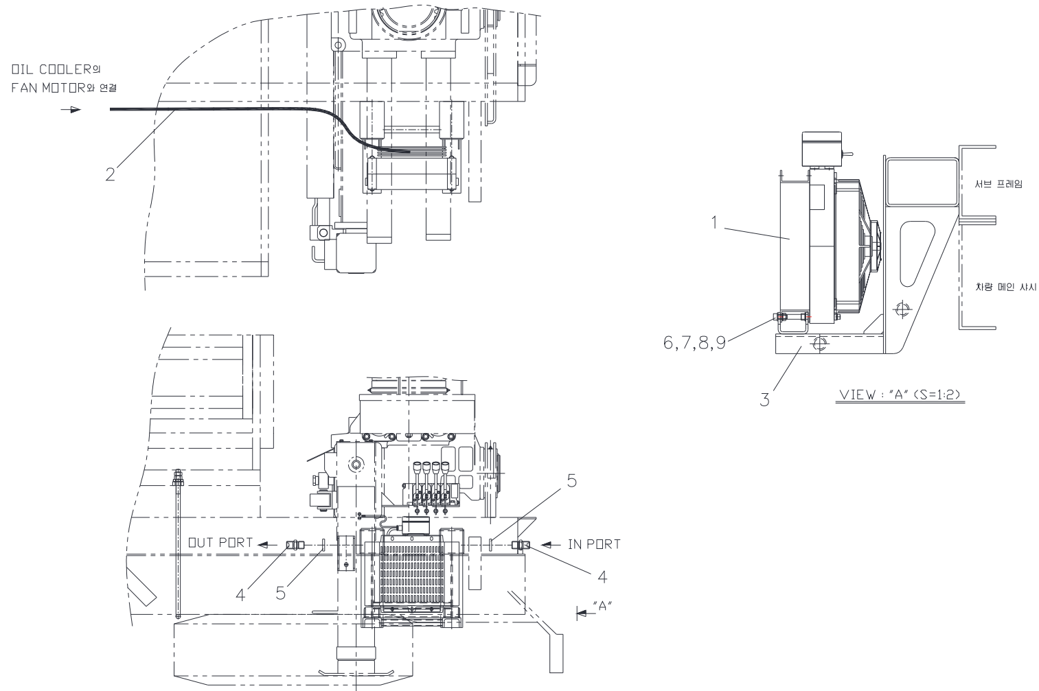
Fig. 7-7 SCK1213 OIL COOLER SET
