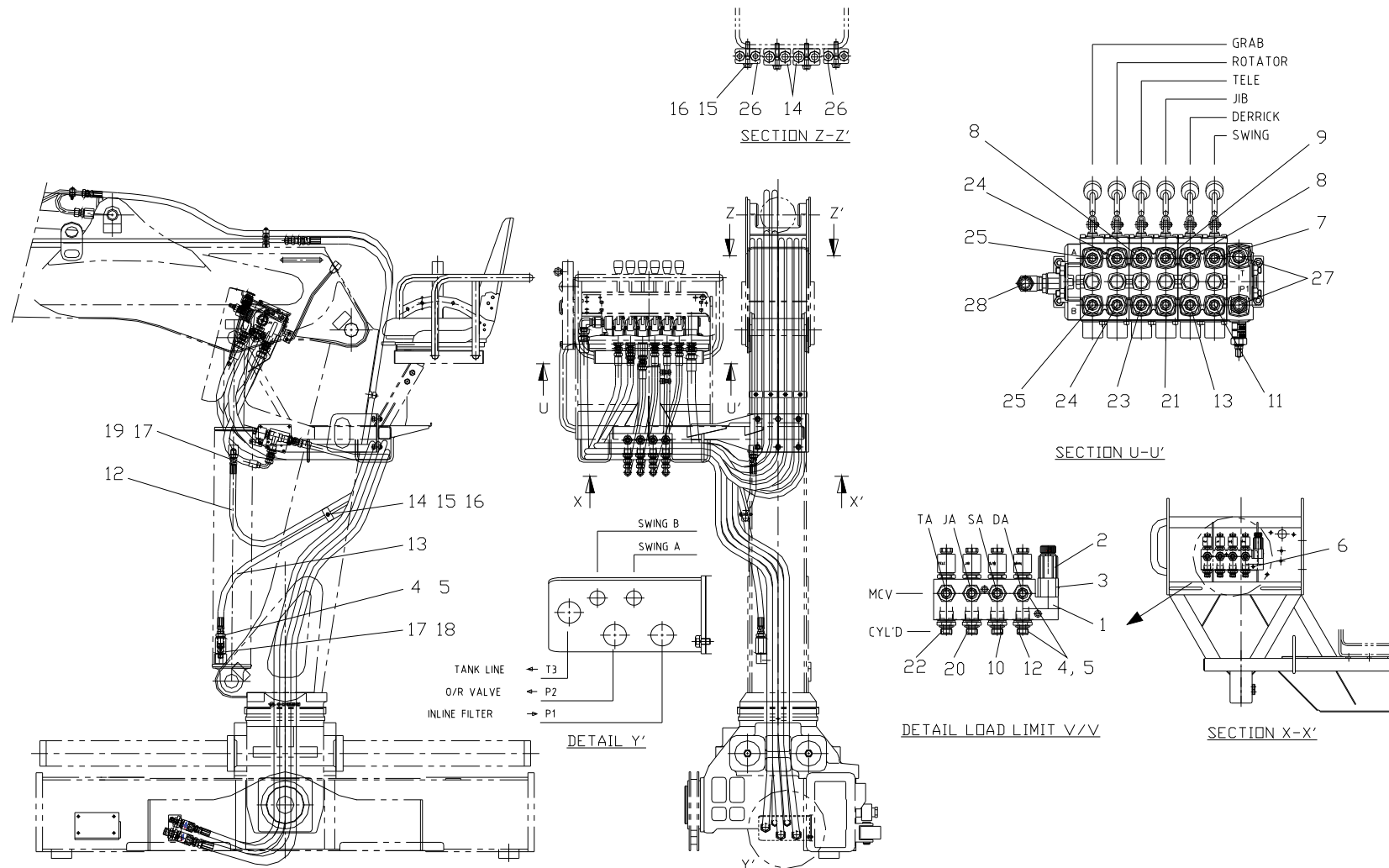
Fig. 4-1 SCK1213 TOP SEAT PIPING
