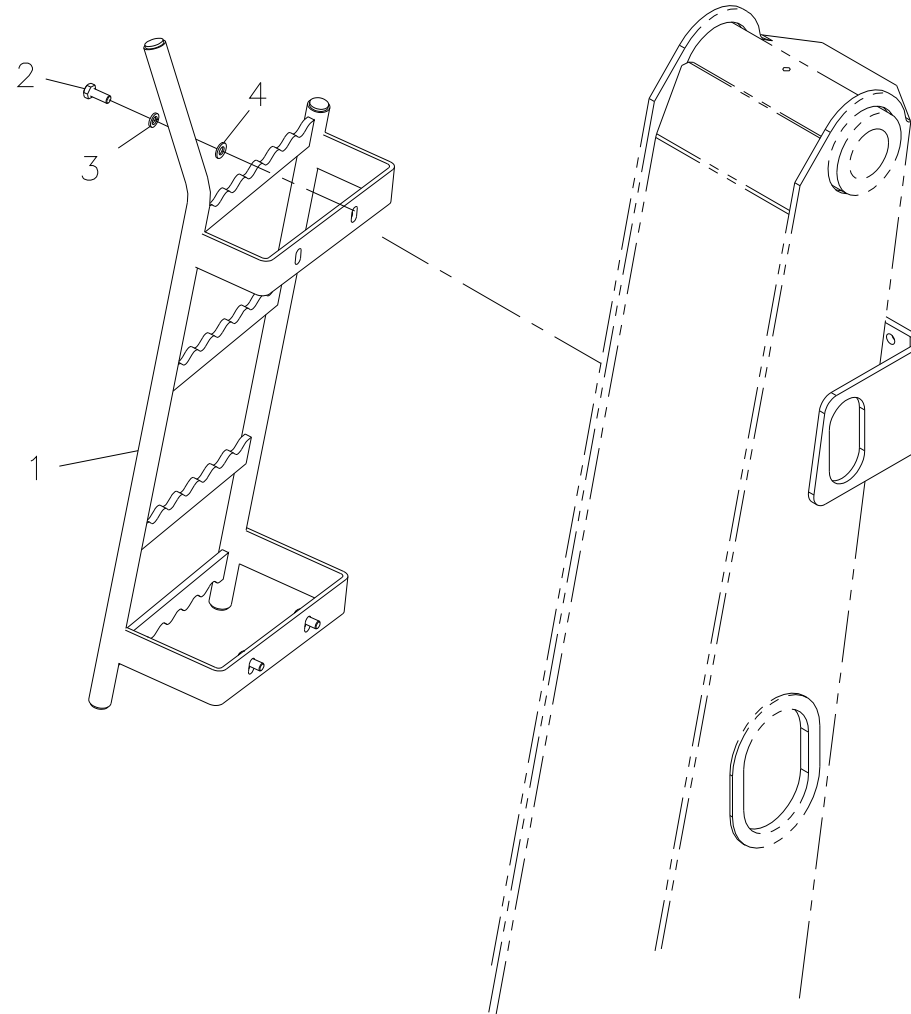
Fig. 2-4 SK11000P LADDER SET
