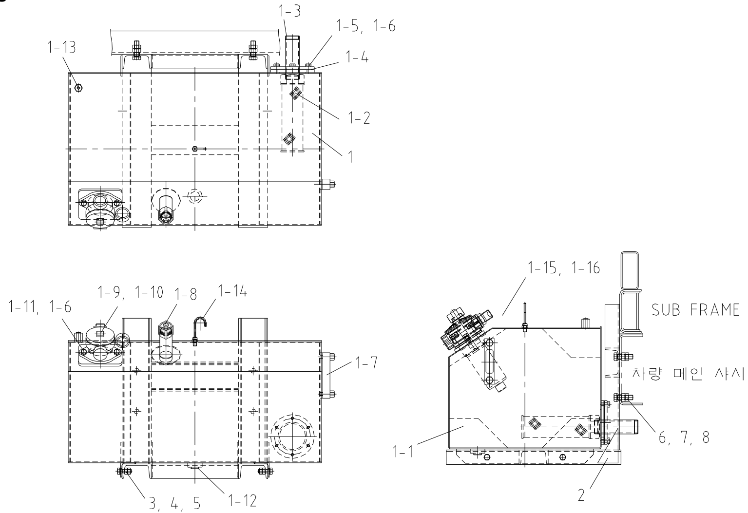
Fig. 7-6 SCK1213 OIL TANK SET
