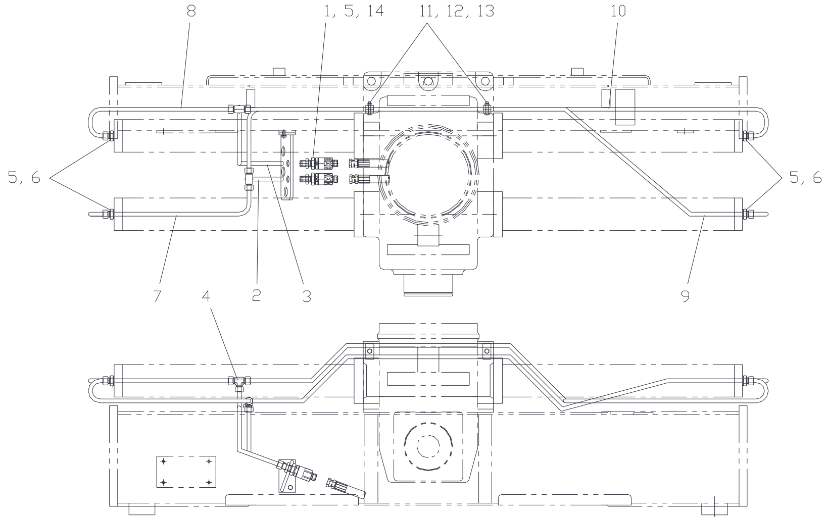
Fig. 4-2 SCK1213 SWING PIPING
