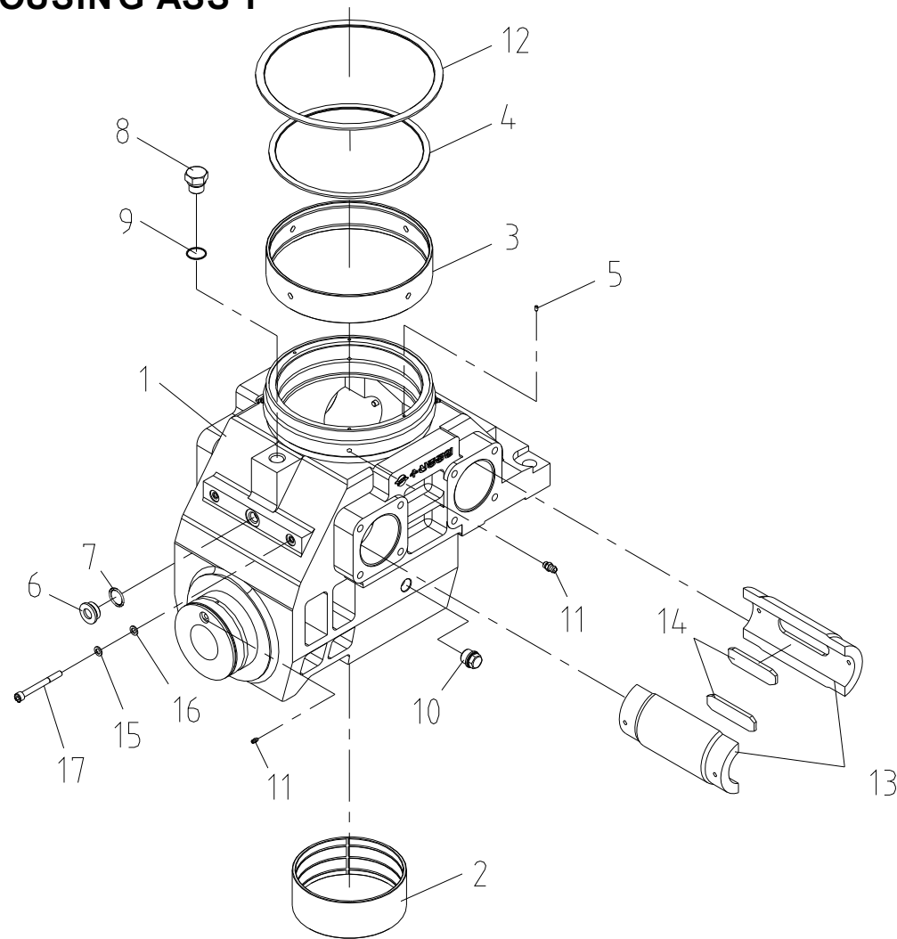
Fig. 2-1-1 SCK1213 HOUSING ASS'Y
