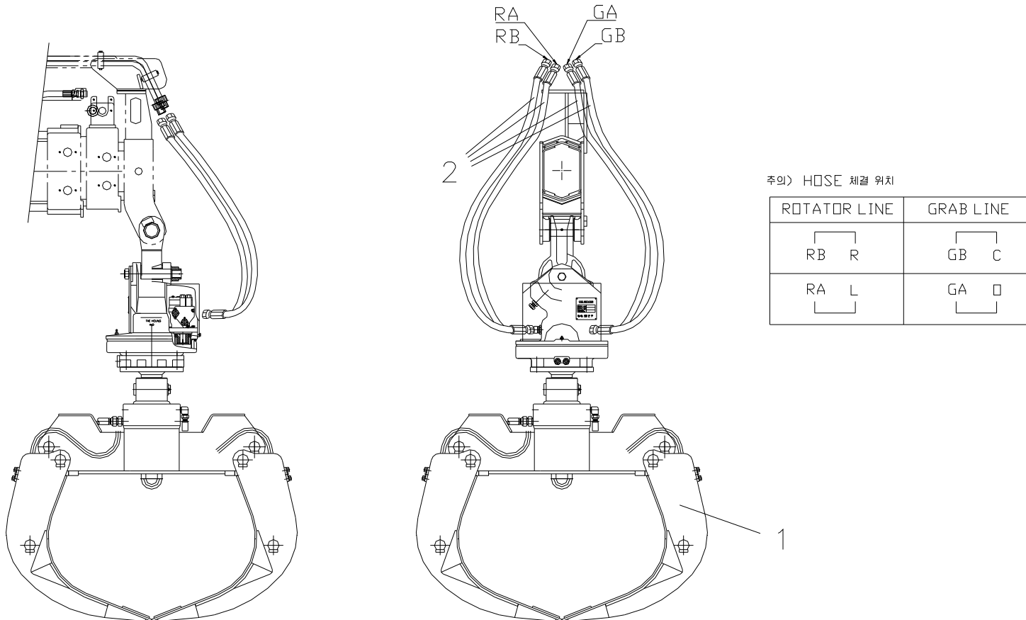
Fig. 6 SCK1213 ATTACHMENT SET
