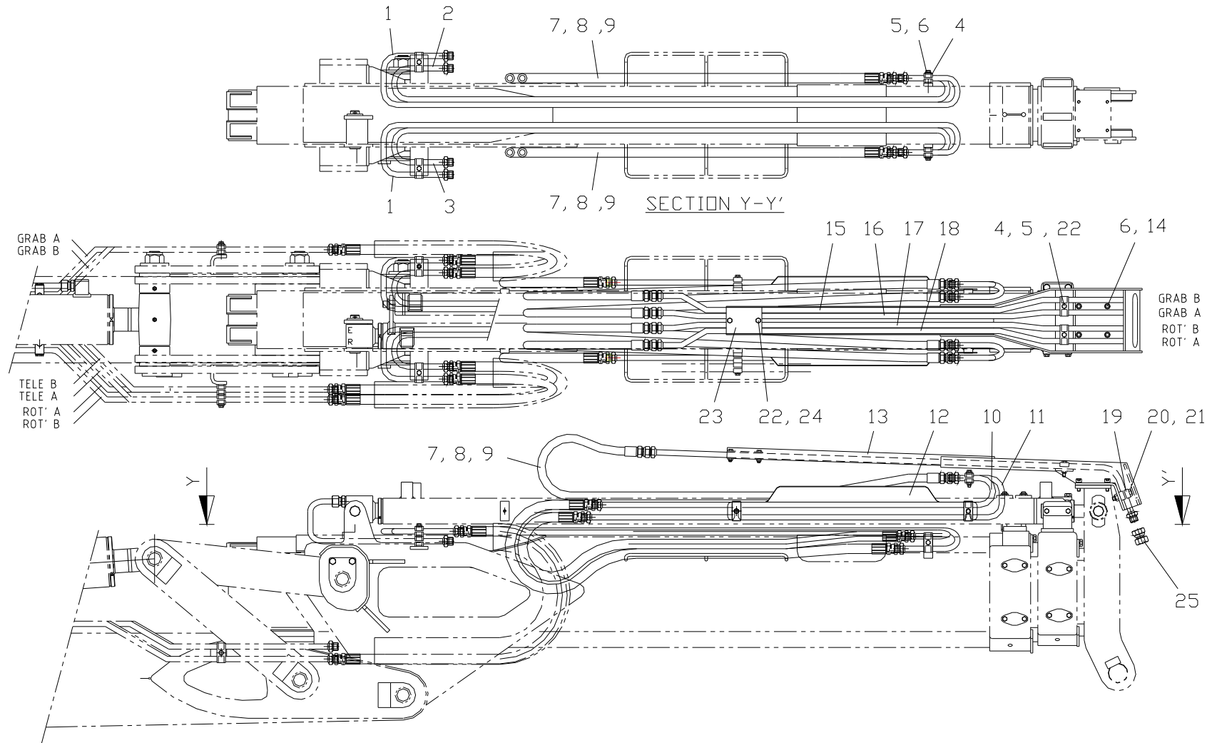
Fig. 4-8 SCK1213 GRAPPLE PIPING
