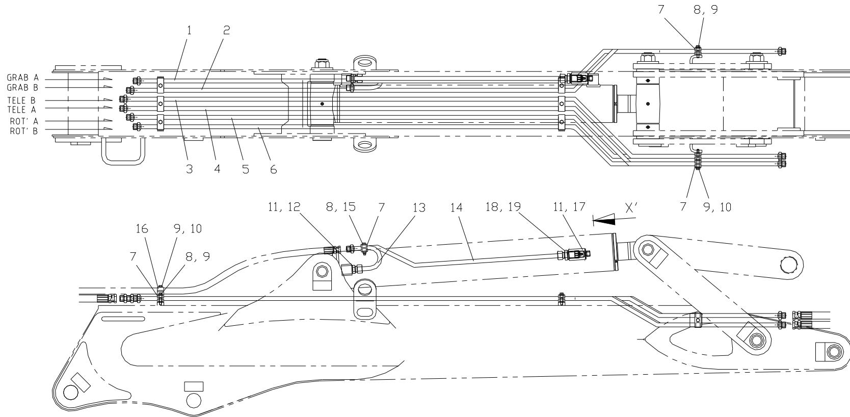
Fig. 4-6 SCK1213 MAIN BOOM PIPING
