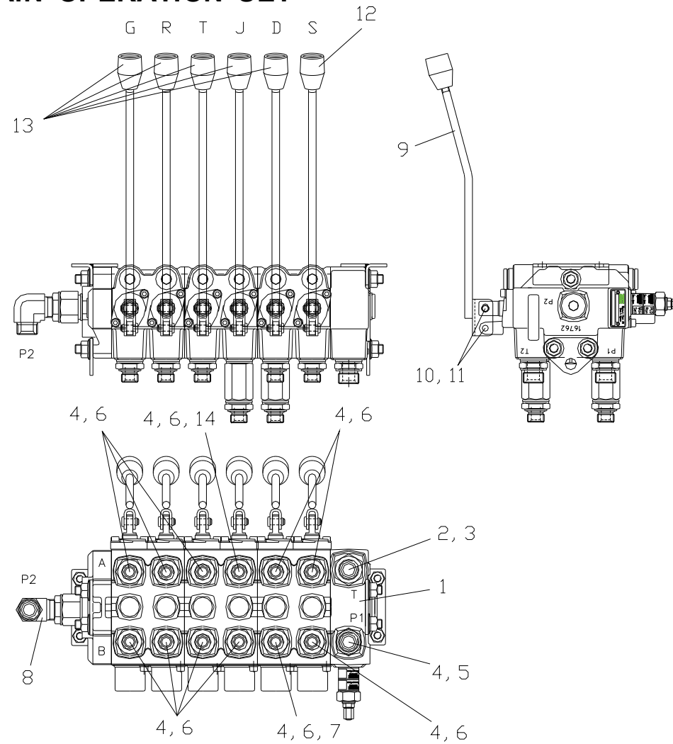
Fig. 3-1 SCK1213 MAIN OPERATION SET
