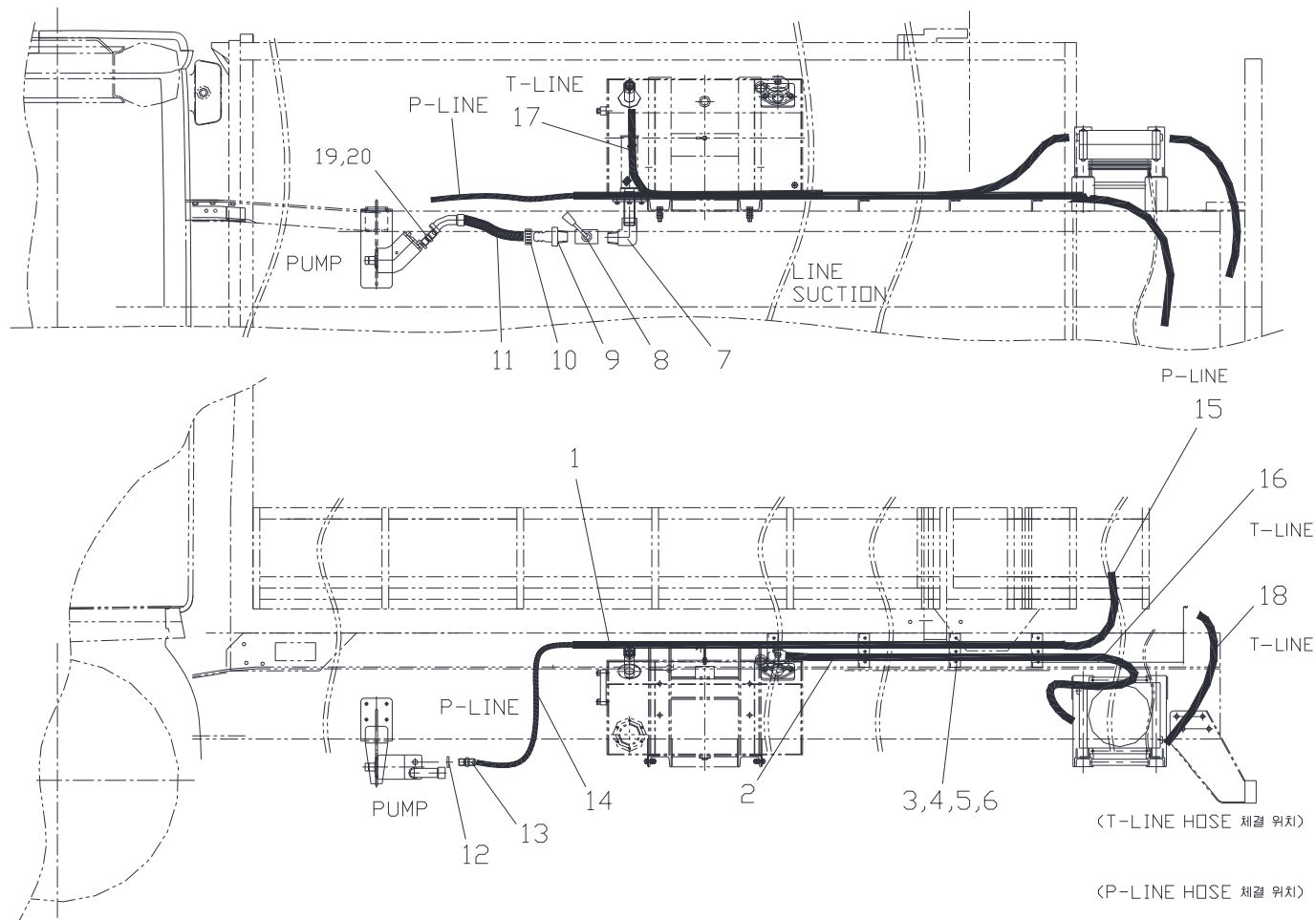
Fig. 7-5 SCK1213 M/ T PIPING SET
