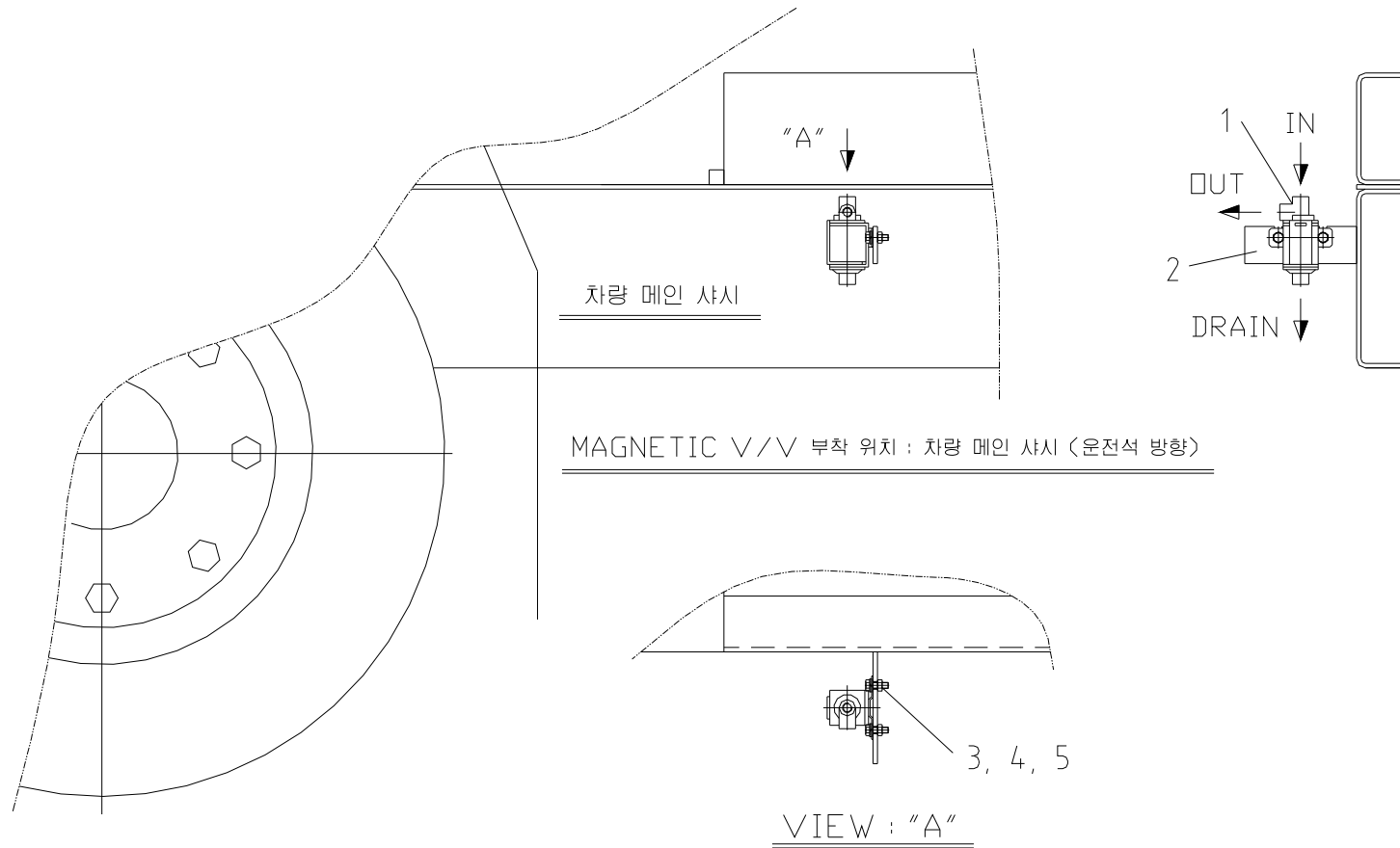
Fig. 7-2 SCK1213 MAGNETIC V/ V SET
