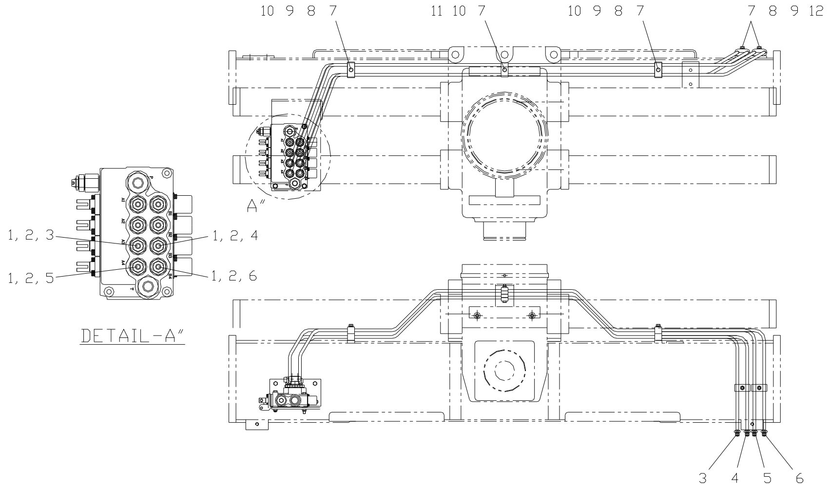
Fig. 4-4 SCK1213 BASE PIPING 2
